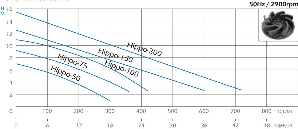
Performance Curve
